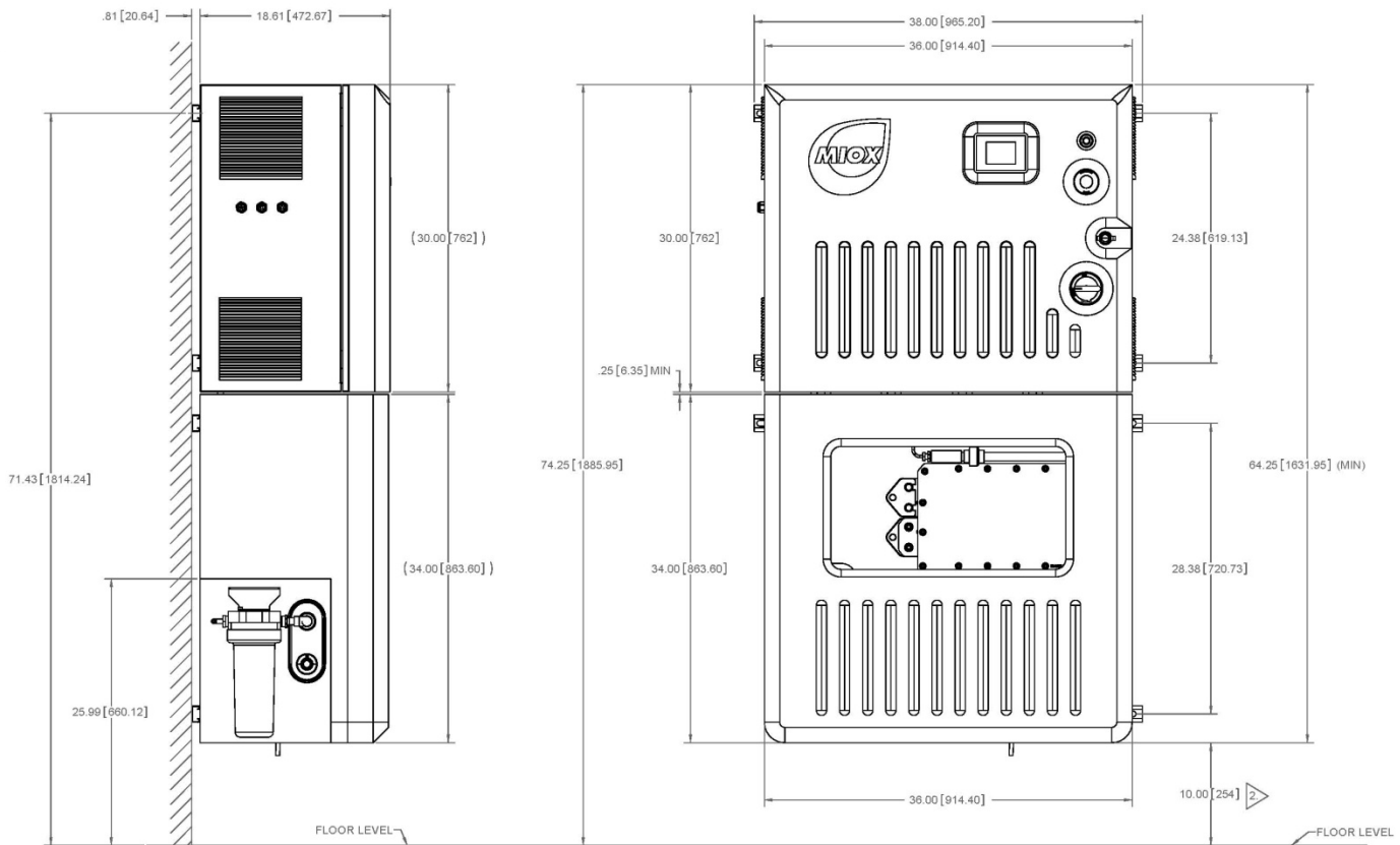
Vault™ Self Cleaning HYPO Drawing
